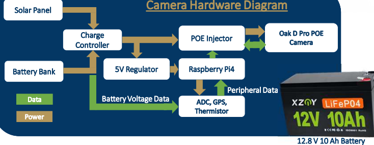
12.8 V 10 Ah Battery
